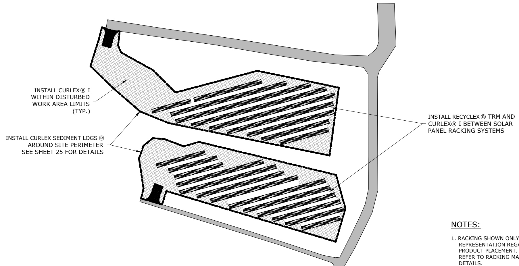
EROSION AND SEDIMENT CONTROL PLAN NO SCALE
