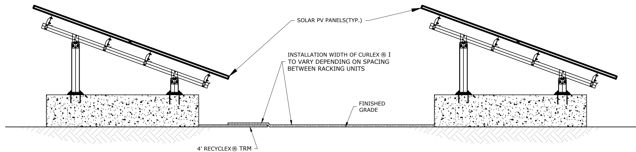
EROSION CONTROL BETWEEN RACKING FOUNDATIONS NO SCALE
