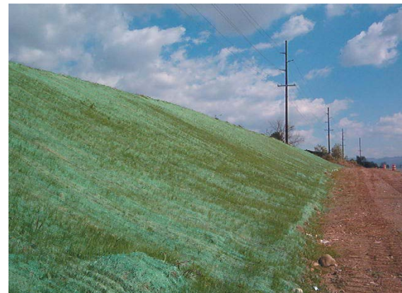
Figure 2. QuickGRASS ® is an aesthetic solution to road side erosion control and revegetation.
