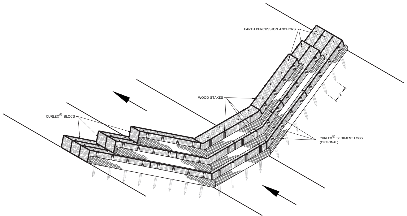
CHANNEL INSTALLATION DETAIL NO SCALE 2 29B
