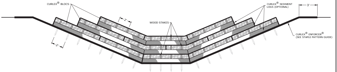
CHANNEL INSTALLATION END VIEW NO SCALE 1 29B
