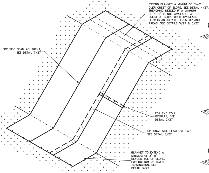
SLOPE DETAIL NO SCALE (1/27)
