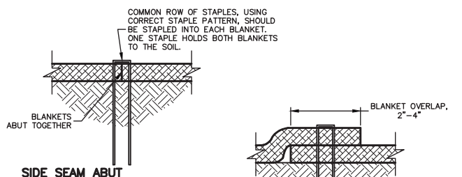
SIDE SEAM ABUT STAPLE DETAIL NO SCALE (7/27)
