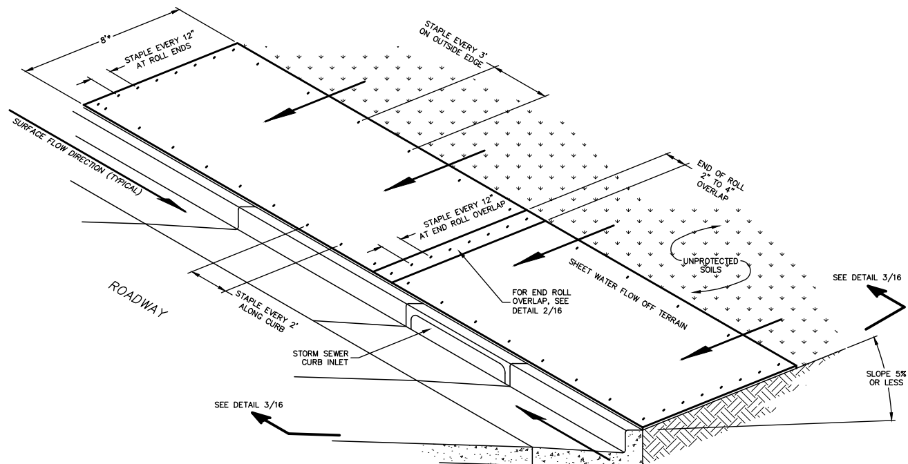
CURLEX® SILTTRAP™ EXCELSIOR BUFFER STRIP NO SCALE
