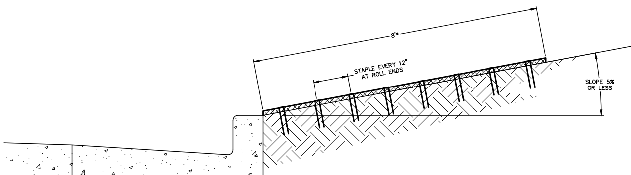
BUFFER STRIP INSTALLATION NO SCALE
