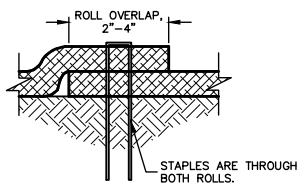
END ROLL OVERLAP STAPLE DETAIL NO SCALE
