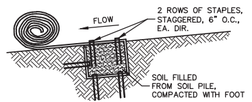
CHANNEL TRENCHING METHOD "A" STEP 1 NO SCALE (8/14)
