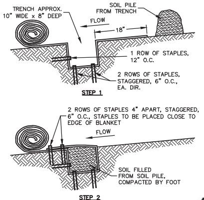
CHANNEL TRENCHING METHOD "B" STEP 1 NO SCALE (9/14)
