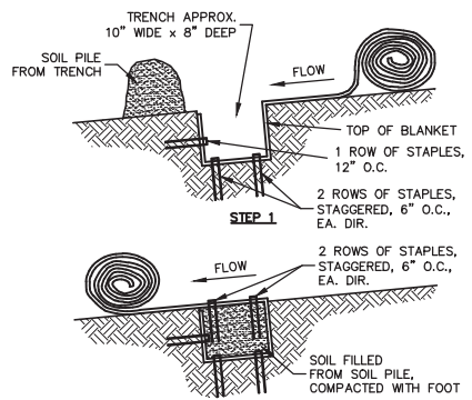
CHANNEL TRENCHING METHOD "A" STEP 1 NO SCALE (8/14)
