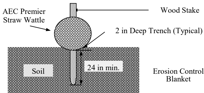
Wattle Cross Section: On Bare Soil
