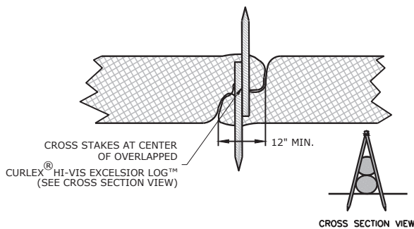
ANCHOR DETAIL (PLAN VIEW) OVERLAPPING JOINT NO SCALE 5 46
