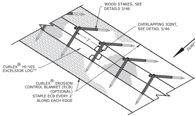
CURLEX ® HI-VIS EXCELSIOR LOG ™ DOUBLED STACKED PROTECTION NO SCALE 1 46
