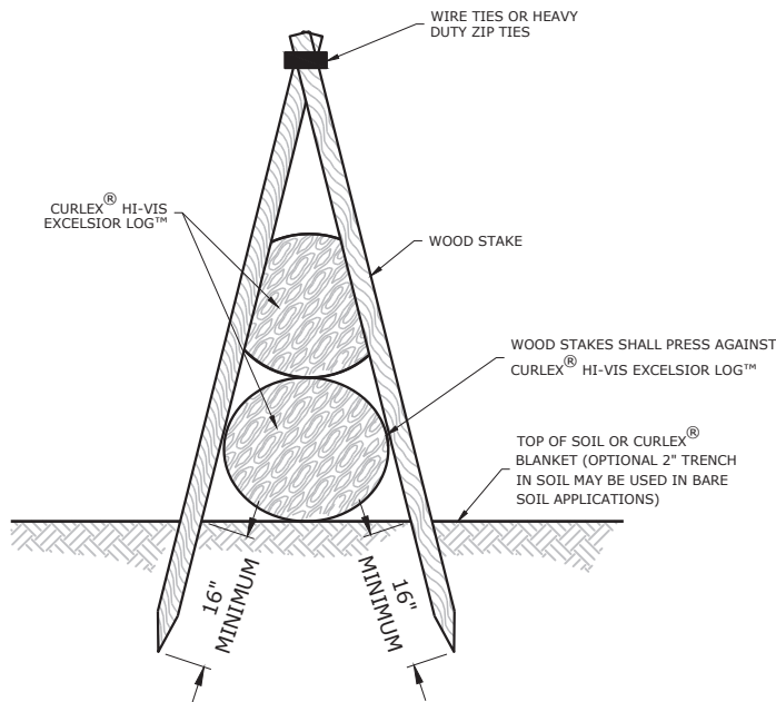
WOODEN STAKES DOUBLE STACKED INSTALLATION NO SCALE 3 46
