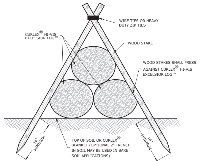
WOODEN STAKES TRIPLE STACKED INSTALLATION NO SCALE 4 46
