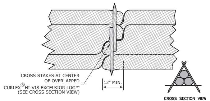
ANCHOR DETAIL (PLAN VIEW) OVERLAPPING JOINT NO SCALE 6 46
