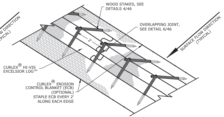
CURLEX ® HI-VIS EXCELSIOR LOG ™ TRIPLE STACKED PROTECTION NO SCALE 2 46
