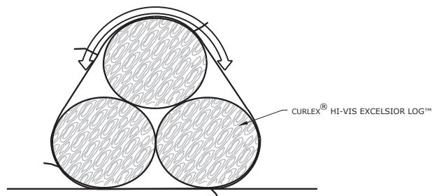
CURLEX® HI-VIS EXCELSIOR LOG™ OPTIONAL STRAP OR WEIGHTED SYSTEM 3 41 NO SCALE
