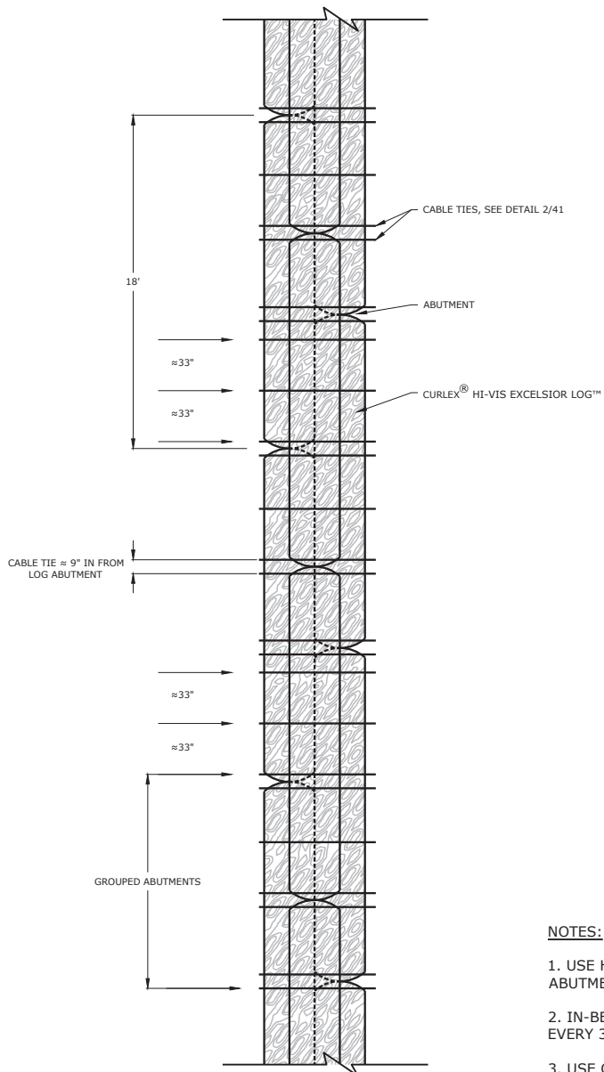
CURLEX® HI-VIS EXCELSIOR LOG™ OPTIONAL STRAP OR WEIGHTED SYSTEM 3 41 NO SCALE
