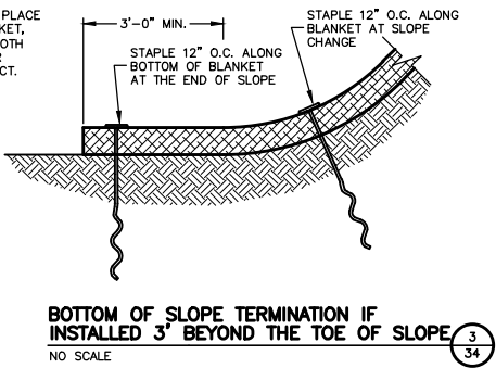
END ROLL OVERLAP NO SCALE
