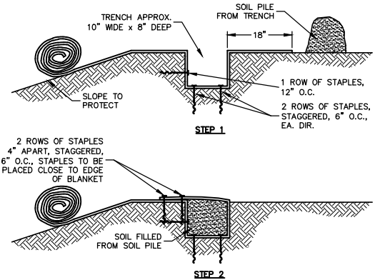
SLOPE TRENCHING METHOD "B" NO SCALE
