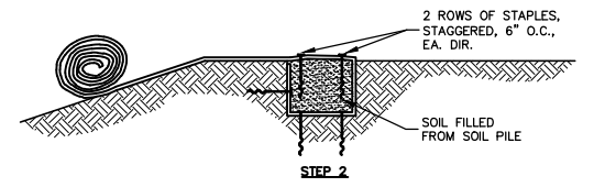
SLOPE TRENCHING METHOD "A" NO SCALE
