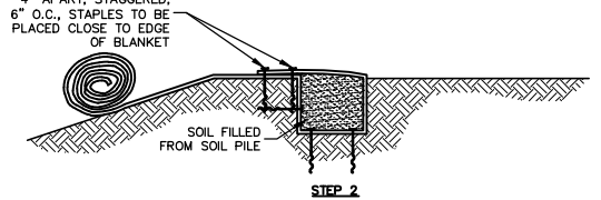
SLOPE TRENCHING METHOD "B" NO SCALE
