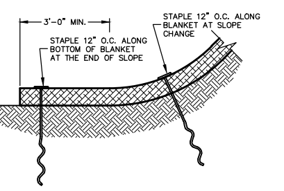
BOTTOM OF SLOPE TERMINATION IF INSTALLED 3' BEYOND THE TOE OF SLOPE NO SCALE
