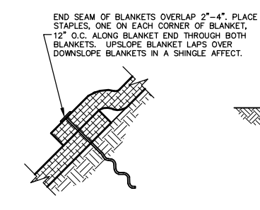
END ROLL OVERLAP NO SCALE
