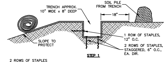
SLOPE TRENCHING METHOD "A" NO SCALE
